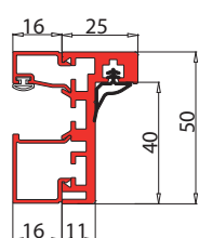
P-088 con/with/mit P-030 or P-031
